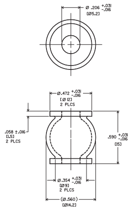
7110 Series Dimensional Drawing
