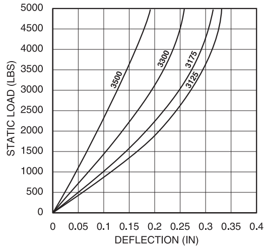
SERIES C, UC 3000 Load vs. Deflection
