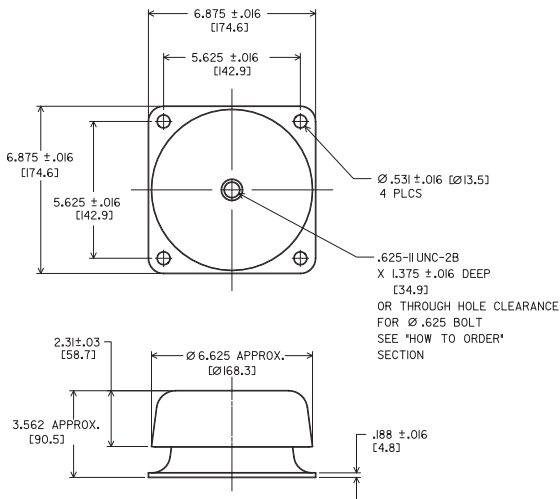
SERIES 3000 Dimensional Drawing
