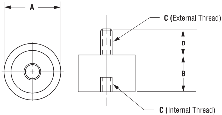
STUD/INSERT (MALE/FEMALE) SERIES Dimensional Drawing (Inches)
