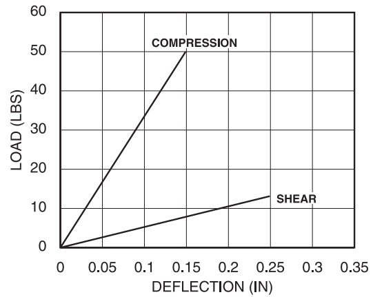
A23-141 Load vs Deflection
