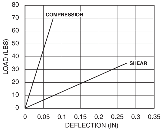
A21-141 Load vs Deflection
