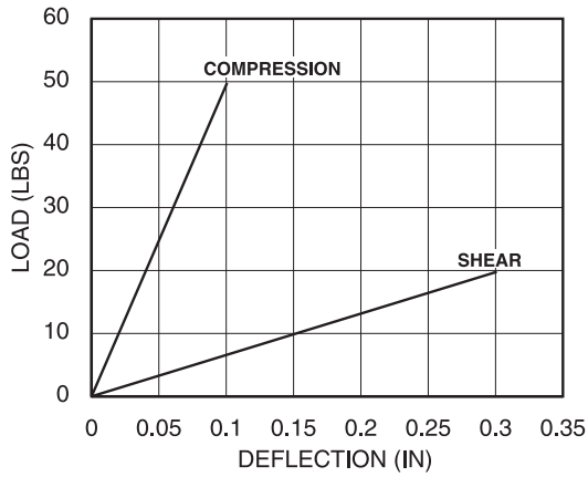
A22-141 Load vs Deflection
